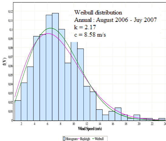
Fig. 5 Probability density distribution of annual wind speeds
