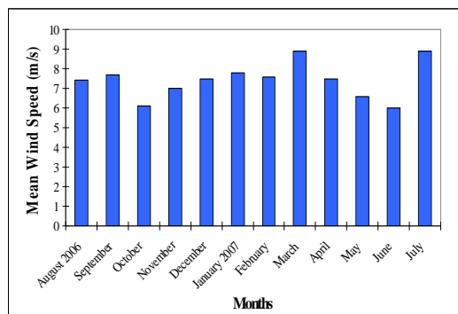
Fig. 1 Monthly mean wind speeds at 10 m height
