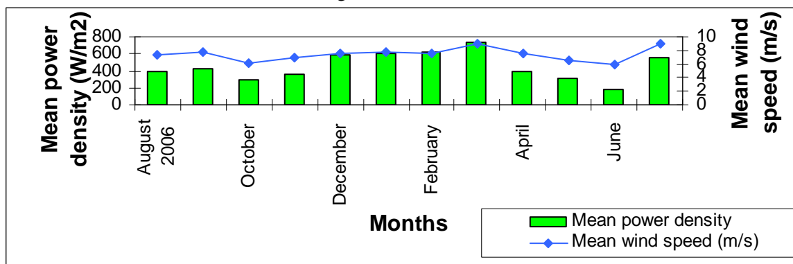
Fig. 4 Monthly variation of the mean power densities and mean wind speed
