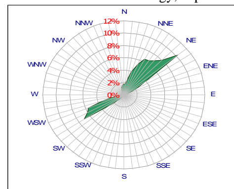
Fig. 3 Annual wind rose based on energy
