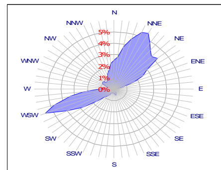
Fig. 2 Annual wind rose based on time
