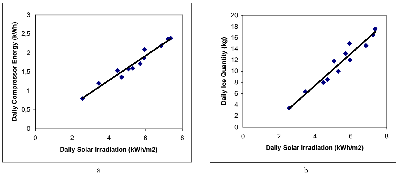
Fig. 4 The performance curves of the ice-maker. a. Energy exploitation, b. Ice formation.
