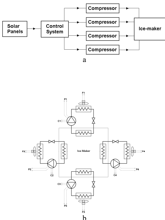
Fig. 1 The ice-maker configuration. a. Block diagram, b. The cooling circuits.
